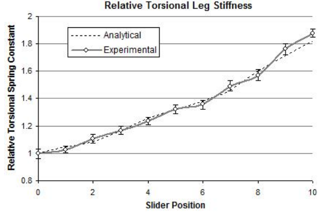
Figure 7. EXPERIMENTAL VALIDATION OF THE PRB MODEL FOR ESTIMATING TORSIONAL SPRING CONSTANT.
