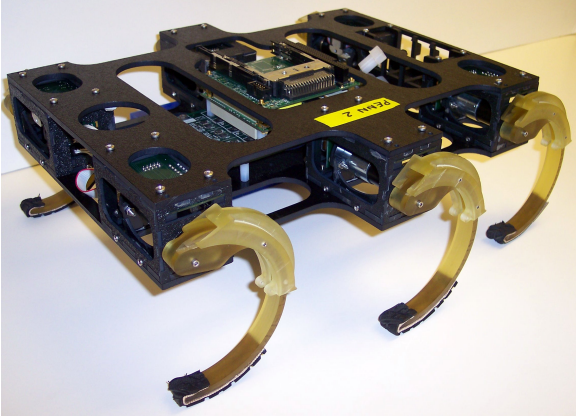
Figure 1. TUNABLE STIFFNESS LEGS ADAPTED TO EDUBOT, A RHEX INSPIRED DYNAMIC LEGGED LOCOMOTION ROBOT.
