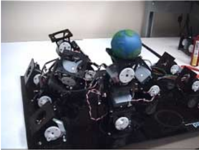
Figure 8: Four arms with three G1 modules each. A small ball is balanced on the end of one arm and passed to the top of an adjacent arm.
